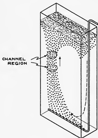
FIG. 2. Path of bubbles rising from a horizontal distributor on the bottom of the tank.
